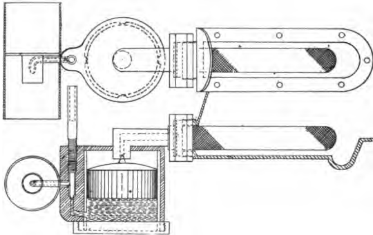
FIG. 316.—The Duryea Float Feed Carburettor or Sprayer.
